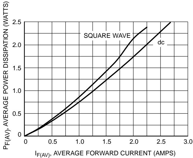
Figure 6. Power Dissipation
